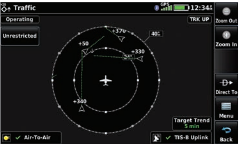
With ADS-B “In” from a compatible receiver (sold separately), the aera 660 and aera 760 can display traffic enhanced with Garmin TargetTrend™ technology, which shows target trajectories relative to your aircraft.
