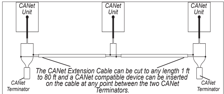
Fishfinder 340C CANet Wiring Diagram
