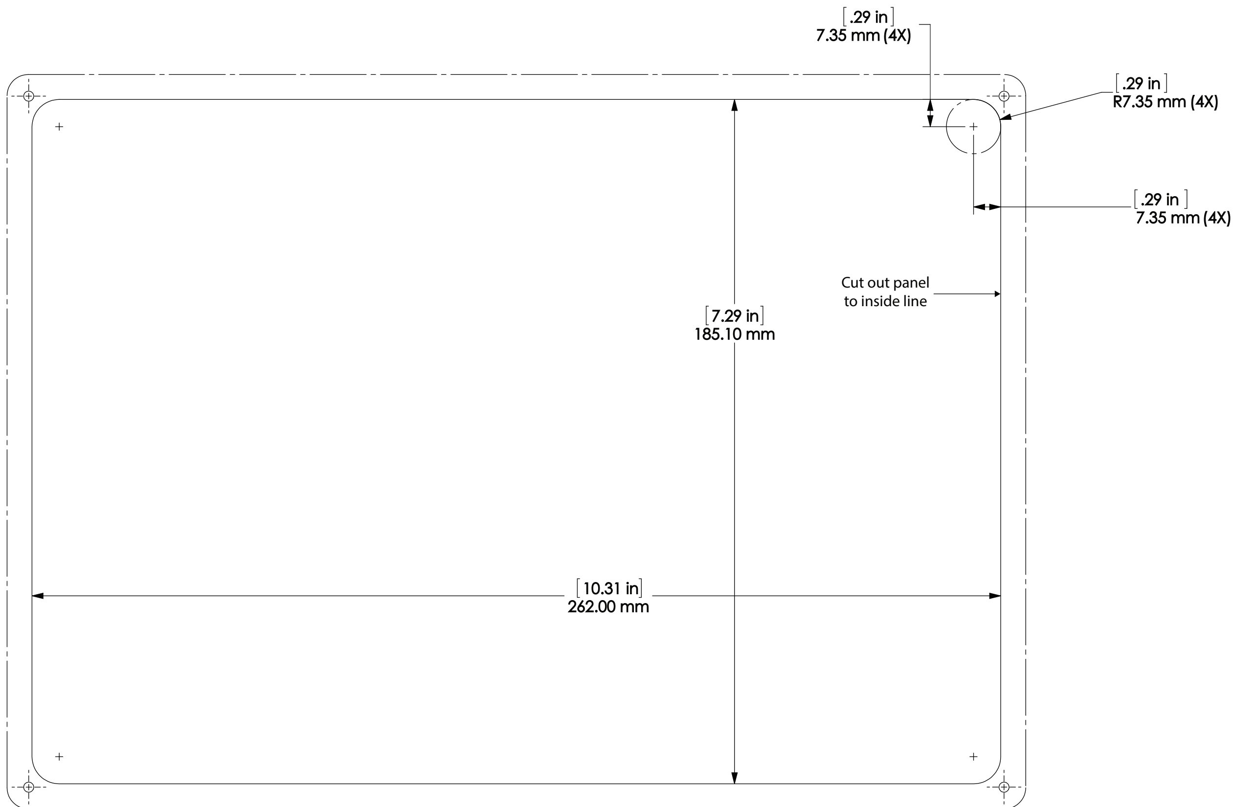
GDU 46X Panel Cutout Drawing
