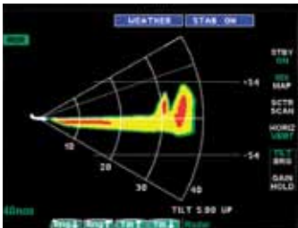
A vertical scanning function on the GWX 68 lets pilots analyze cloud tops and storm gradients to see a more complete weather picture.
