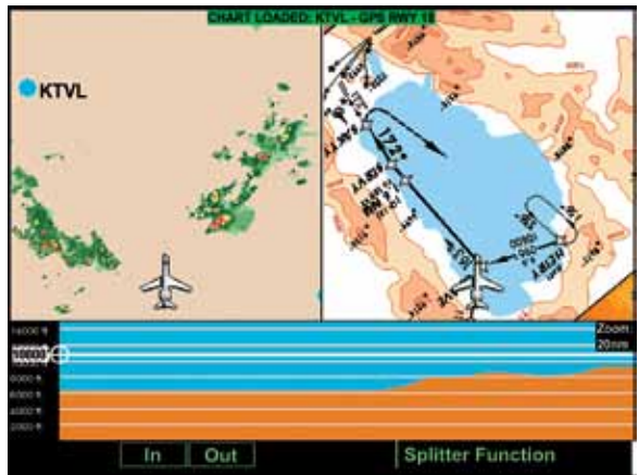
For added situational reference, the latest GMX 200 software offers a unique split-screen view – allowing side-by-side displays of any two GMX 200 charting functions. In addition, a vertical profile view of terrain peaks and obstructions relative to the current flight level can be displayed across the lower portion of the screen.
