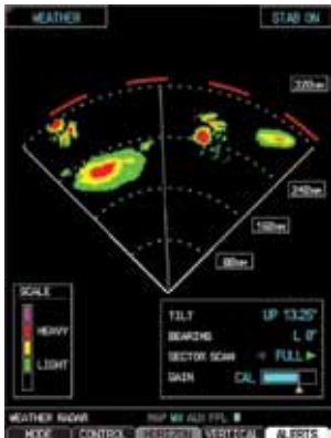
Garmin's WATCH™ weather attenuation feature highlights areas where radar energy may be partially absorbed by precipitation and, thus, not fully reflect storm intensity. The radar interface is included with the G600 system, an optional enabling card is available for the G500.
